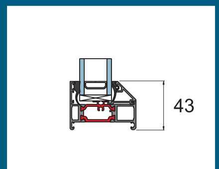
Bottom Detail Fixed Lite
