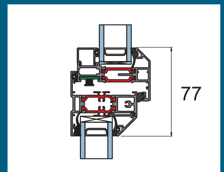
Chelton Vent / Transom Detail
