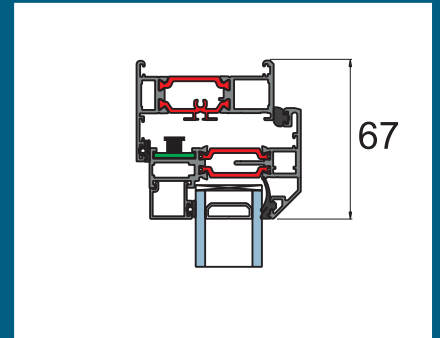
Chelton Vent / Head Detail
